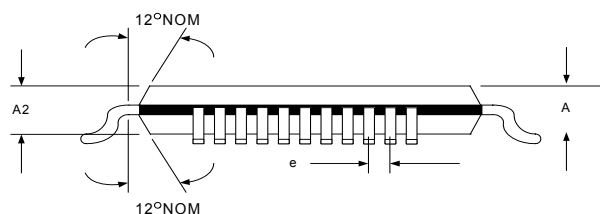
Figure 4 - LQFP-100
