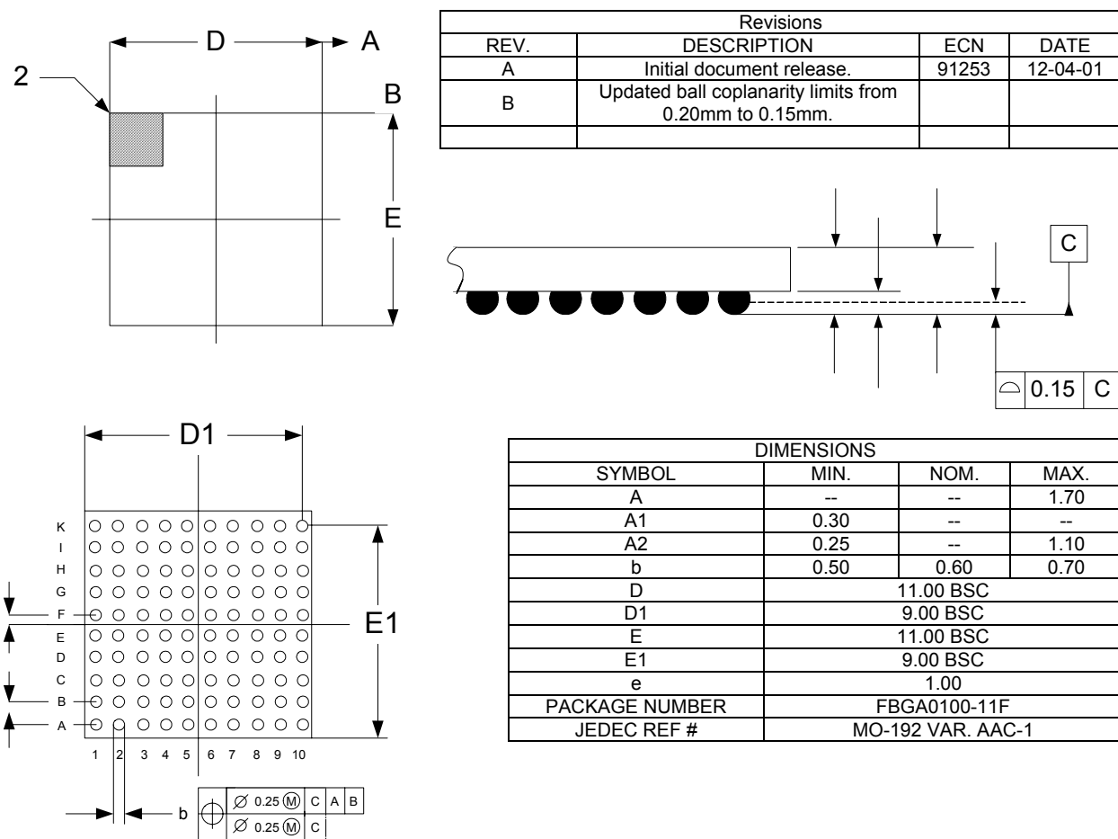
Figure 5 - FPBGA-100
