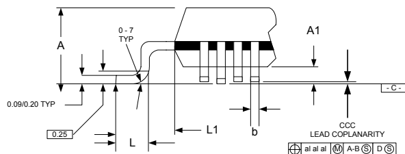
Figure 4 - LQFP-100
